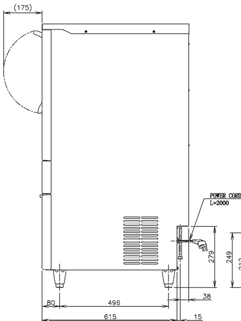
RIGHT SIDE
