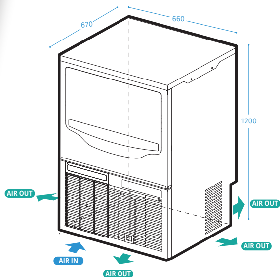
FRONT SIDE
